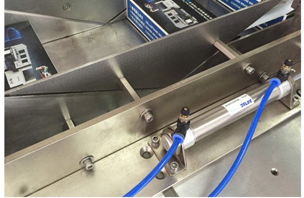
Carton transfer detail
