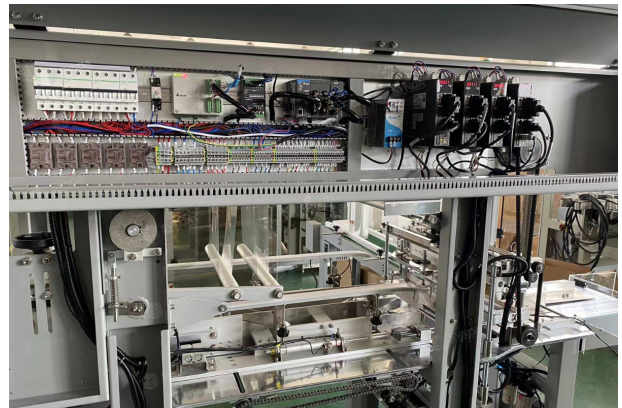
Internal mechanism
