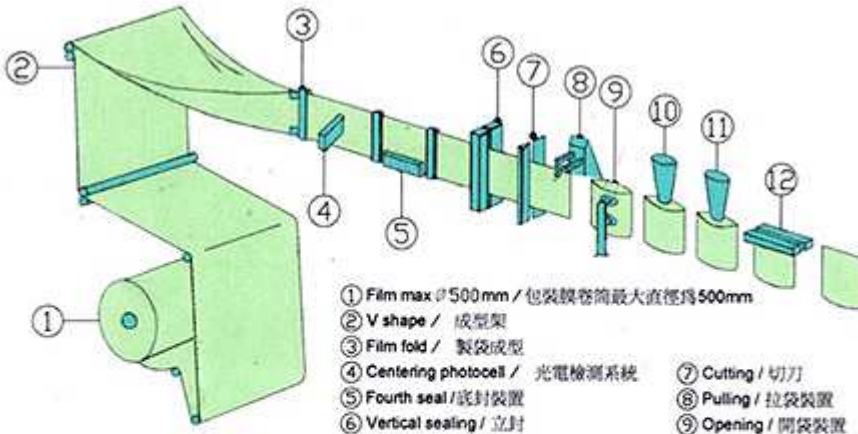
双袋三邊封 Two bags three side seal
