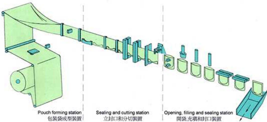
双袋一連 Two bags one string
