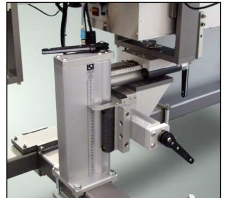
Rigid XYZ Head Mounting w/ 2 Axis Fine Adjustment to repeatable and accurate labeling.
