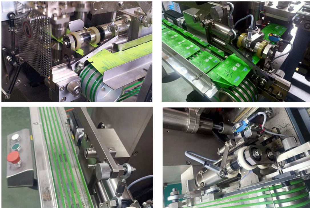
STB-120 High-Speed Tea-Bag Envelope Packing Machine Details
