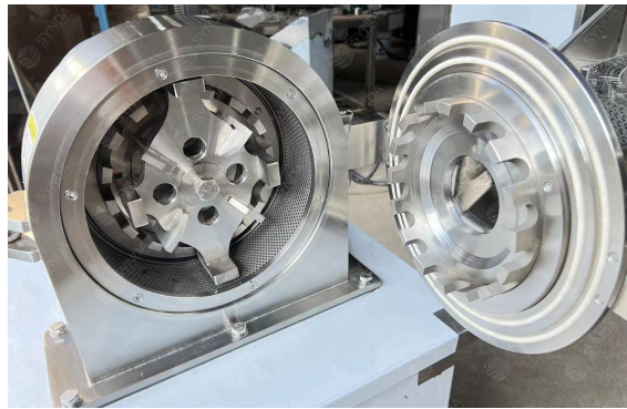
G20B Tea Grinding Machine Details
